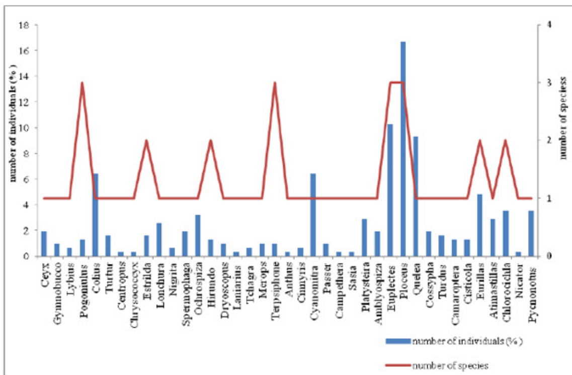
Fig. (3). Histogram of the relative abundances of the genera captured in the Abobo-Etetak hill and species number curve.
